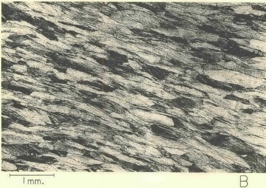
PHOTOMICROGRAPHS OF HIGHLY DEFORMED YULE MARBLE
